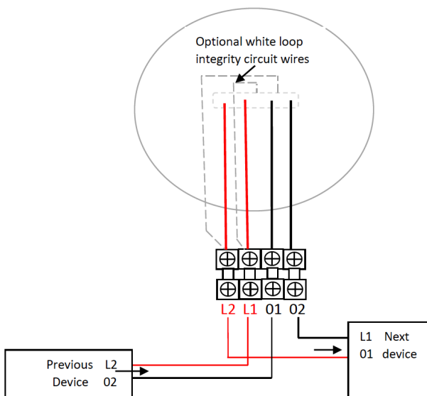
CEILING DISK A Diagram 1
